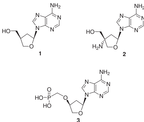
FIGURE 1 Examples of apiosyl nucleoside analogues as potent antiviral agents.
