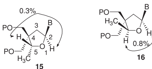
FIGURE 2 NOE comparisons of compounds 15 and 16 .
