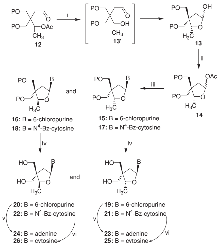
SCHEME 2 Synthesis of target nucleosides. Reagents: i) NaOMe, MeOH; ii) Ac 2 O, DMAP, pyridine; iii) persilylated bases, TMSOTf, ClCH 2 CH 2 Cl; iv) TBAF, THF/CH 3 CN; v) NH 3 /MeOH, steel bomb, 90°C; vi) NH 3 /MeOH, room temperature.
